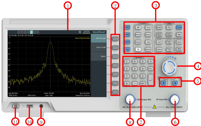
Figure 3- 1 Front panel
