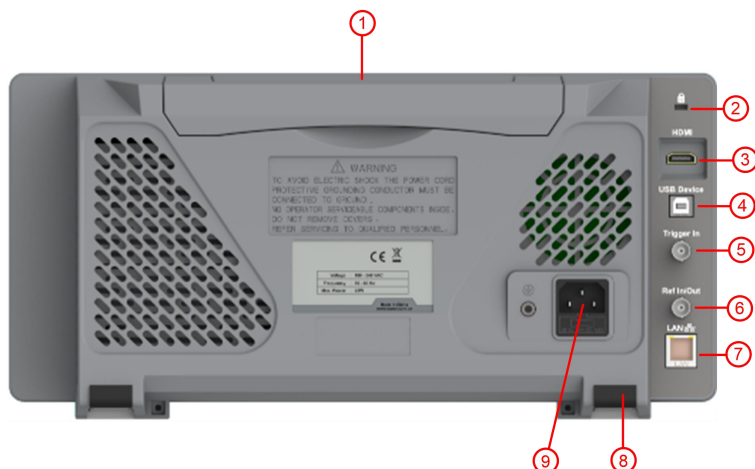
Figure 3-6 Rear Panel
