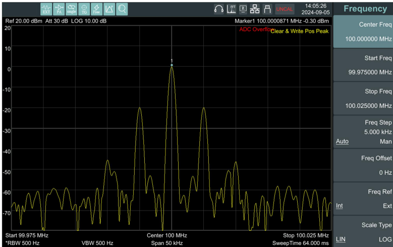
Figure 3- 8 Full Span
