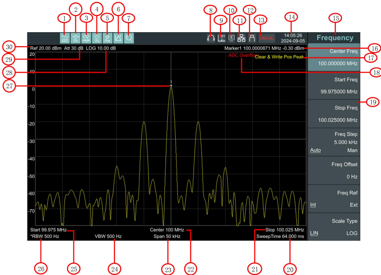
Figure 3-7 User interface
