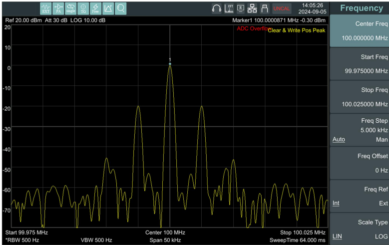
Figure 3-9 Set frequency span
