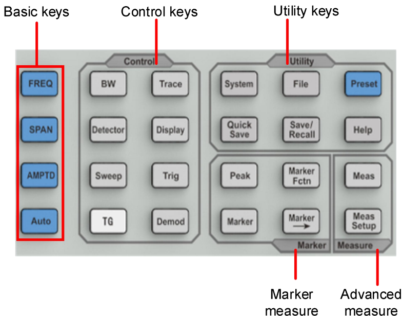
Figure 3-2 Function Keys
